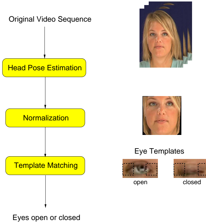
Figure 4.9: Block diagram of automatically detecting eye blinks. Before normalizing the head pose is estimated. Afterwards a template matching based on two templates indicates whether the eyes are opened or closed. As templates both eye corners are used (indicated by the black dashed rectangle).
