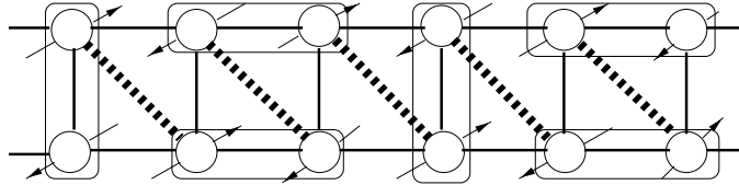
FIGURE 2.2: Typical configuration in the RVB state of AFM ladder
