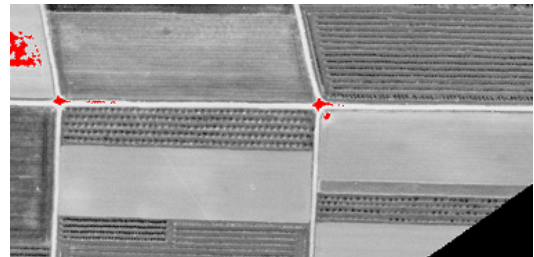
Figure 5. Out-of-sample test with 30 degree rotated image (the training was executed with no rotation)
