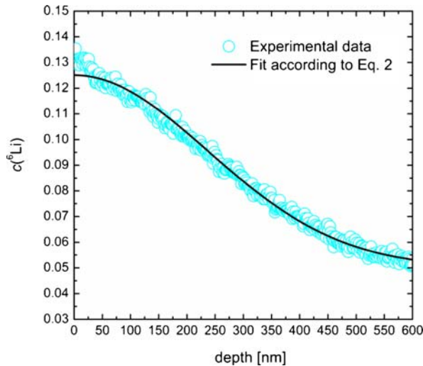
Fig. 5. Atomic fraction of 6 Li as a function of depth after annealing at 383 K for 2 min. A least-squares fit of Eq. (2) to the experimental data is also shown ( h = 24 nm, R = 327 nm).
