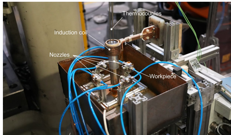
Fig. 3. Experimental setup of the heating unit with spray nozzles.
