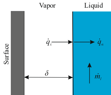
Fig. 1. Leidenfrost scheme demonstrating formation of a vapor layer.
