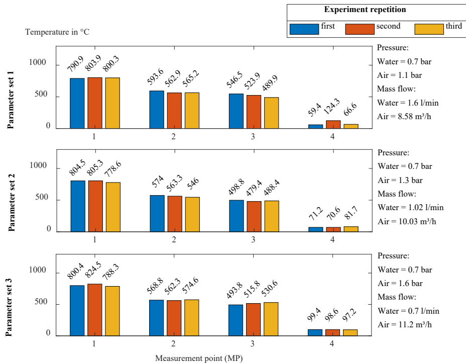
Fig. 5. Bar plot of the experimental results showing the maximal measured temperatures for each parameter set and repetition.
