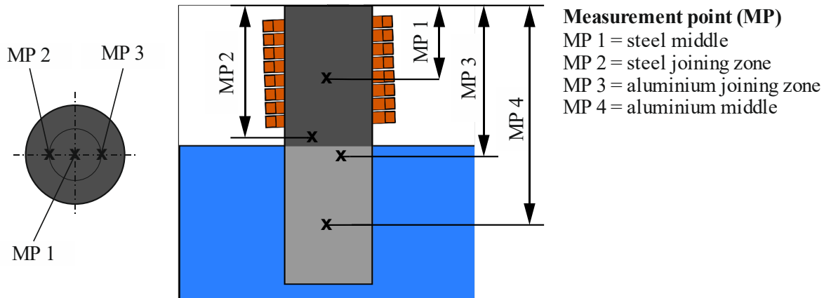
Fig. 2. Scheme of immersion cooled shaft workpiece during inductive heating with marked measurement points (MP).
