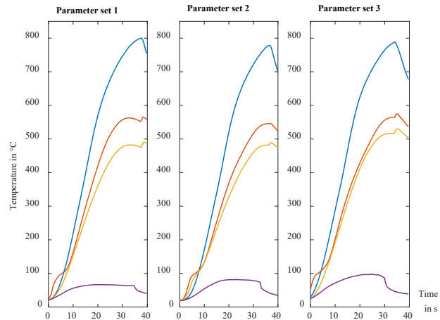
Fig. 4. Temperature in different measurement point (MS) during inductive heating and simultaneous spray cooling.
