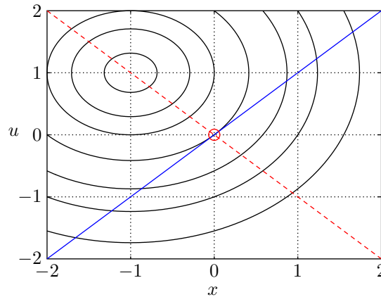
FIGURE 1. Illustration of the steady-states (blue solid line), level sets of \ell (black ellipses), and the additional constraint g_{ad} (red dashed) of the example in Section 8.4. The optimal steady-state (x^e, u^e) = (0, 0) for the undiscounted case is marked with a circle.
