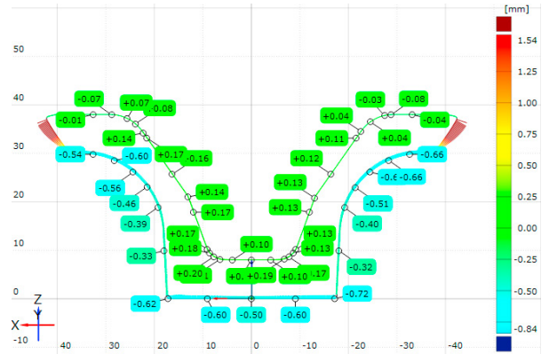
Fig. 3. Deviations measured on a forged part ( T_{1,7225} = 1250^{\circ}\text{C} ; T_{1,2714} = 250^{\circ}\text{C} ) using GOM.
