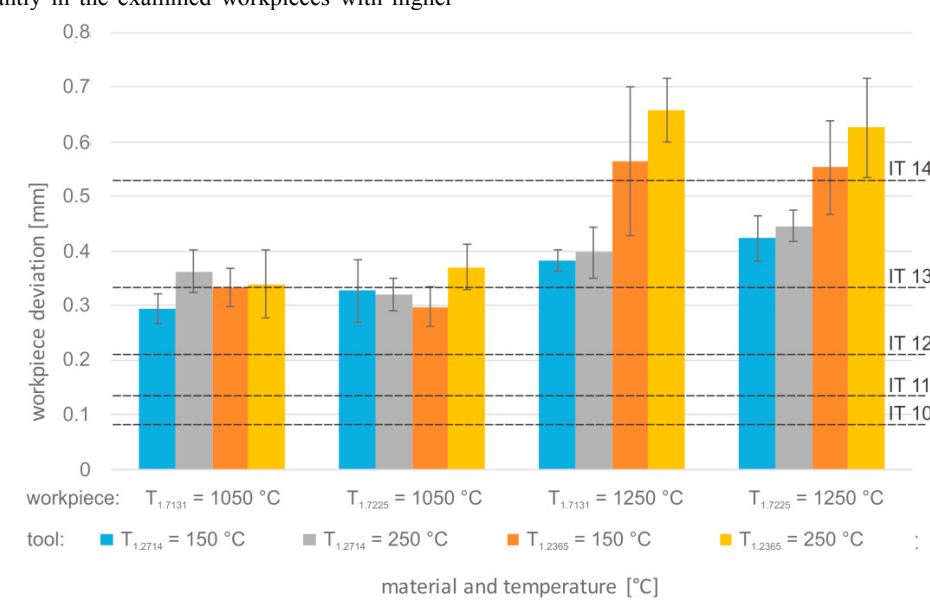
Fig. 5. Arithmetic mean of the measured deviations on forged workpieces under varied tool and workpiece material at different interacting temperatures.
