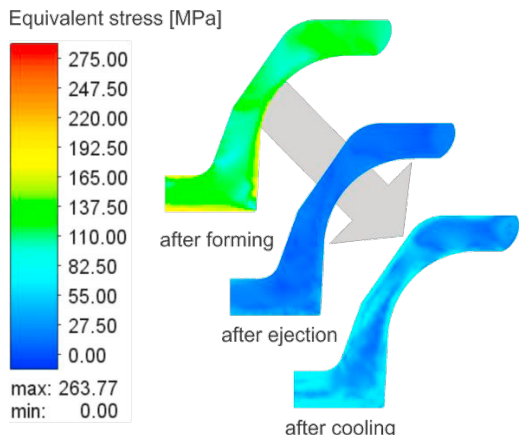
Fig. 4. Equivalent stress of the part in the process stages after forming, after ejection and after cooling to ambient temperature (tool: 1.2714 - 250°C; workpiece: 1.7225 – 1250 °C).
