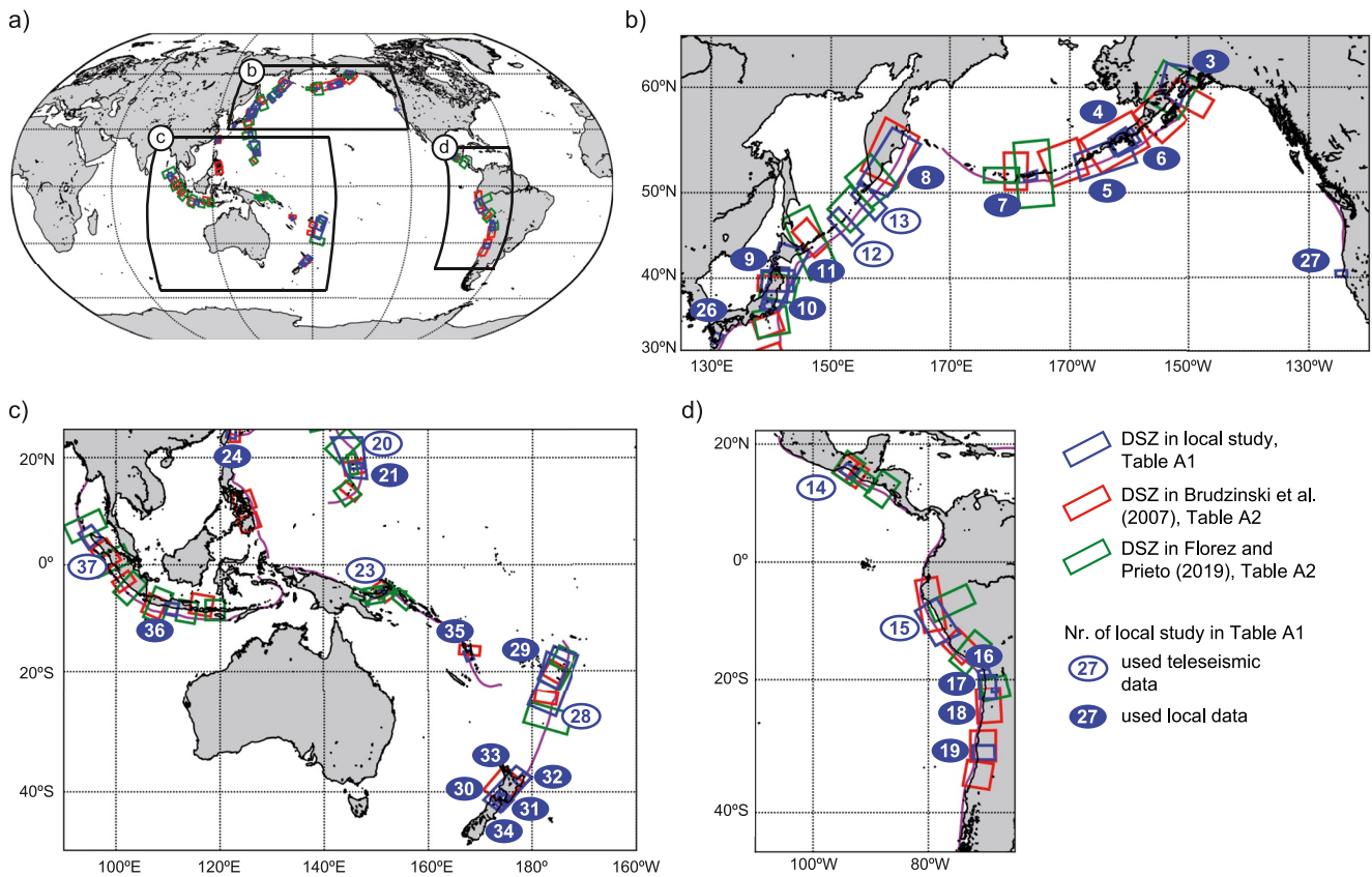
Figure 2. Locations where double seismic zones have been postulated in local studies (blue rectangles) and the global studies of Brudzinski et al. (2007) (red rectangles) and Florez and Prieto (2019) (green rectangles). For details and references, refer to Tables A1 and A2. Magenta solid lines mark trench locations.
