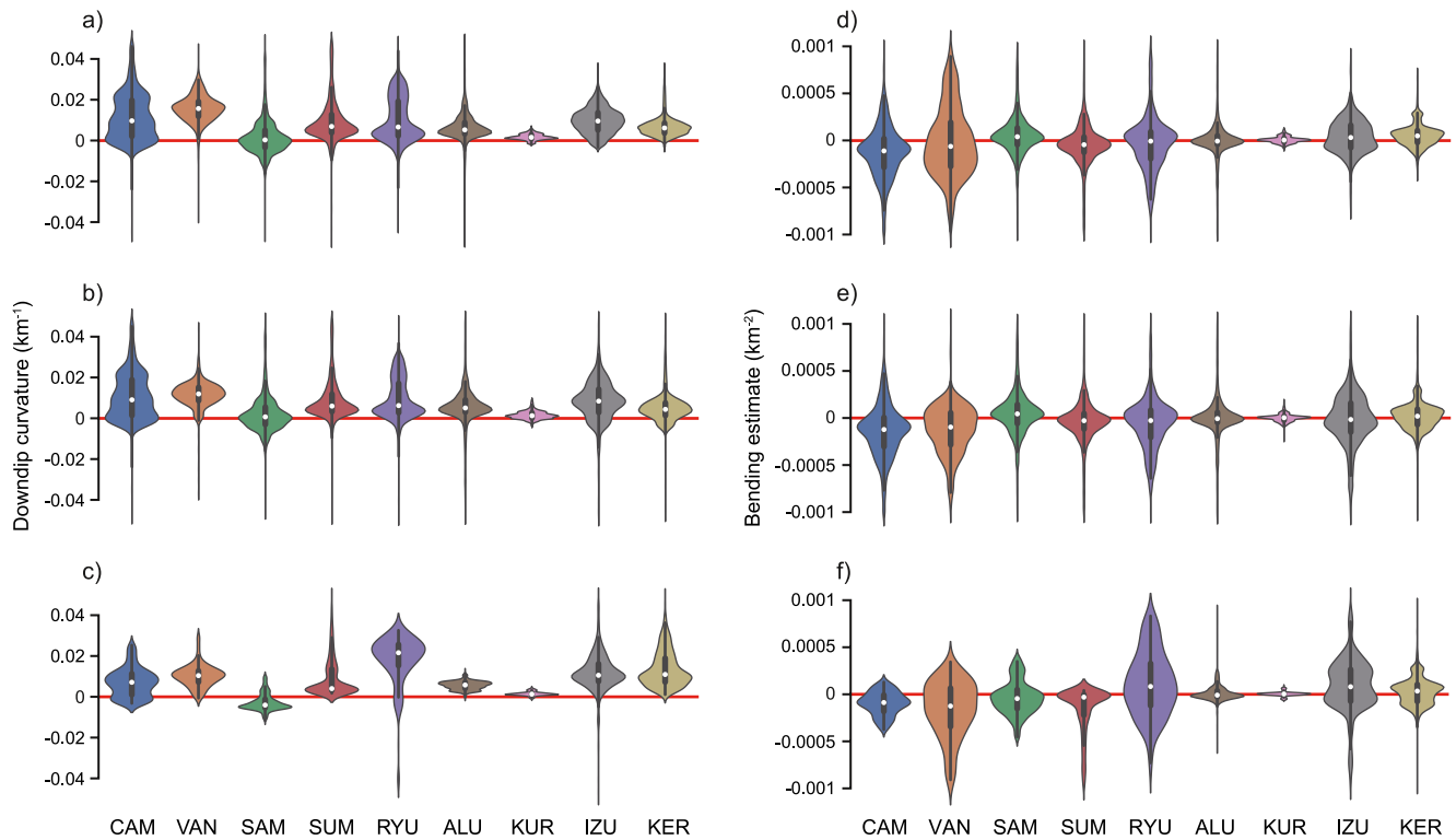
Figure 6. Summary of slab curvature values (left column) and bending estimates (right column) derived from slab2 grids, for different slabs in depth intervals that are associated with double seismic zone (DSZ) seismicity. The violin plots summarize the frequency of occurring curvature data points (negative values correspond to upward curvature, positive values to downward curvature; see Figure 5). The small white dot in the center of each violin is the median of the distribution, the thick black line marks the extent of the inner quartile range, the thin black line extends another 1.5 inner quartile ranges. The outline of the violin shows the entire distribution of the data. Subfigures (a) and (d) show violin plots for the nine slabs in the depth range of 50–150 km. In subfigures (b) and (e), the investigated depth range is the depth range of actual DSZ earthquake observations (see Table A1) in each subduction zone. In subfigures (c) and (f), finally, only the parts of each slab that fall into the regions of DSZ observations (blue frames in Figure 2) are analyzed, and for each such region the depth range is limited to the depth interval in which DSZ earthquakes have been observed (see Table A1).
