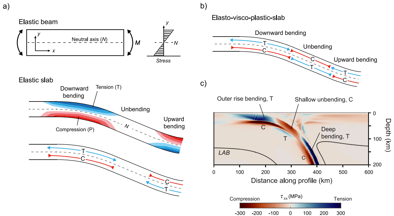
Figure 9. (a) Sketch illustrating the approximation of a slab as an elastic beam. Upward or downward bending of an elastic beam due to a bending moment M causes elastic flexural stresses that linearly increase with distance from the neutral line. For an elastic slab, unbending beyond the outer rise results in a relaxation of stresses. (b) Sketch illustrating the distribution of compression (C) and tension (T) for bending and unbending of an idealized elasto-visco-plastic slab. Note that unbending does not result in stress relaxation as in the elastic case, but a stress reversal. (c) Stress field representation from a numerical modeling study (taken from Bessat et al., 2020), where a transition from outer rise bending to shallow unbending was retrieved, followed by another stress field reversal toward deeper bending at around 120 km depth.
