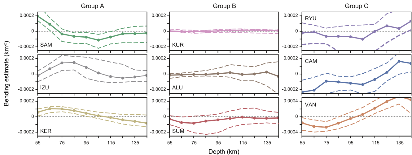
Figure 8. Distribution of bending (values \geq 0 ) and unbending ( \leq 0 ) datapoints in 10 km depth bins in the depth interval 50–150 km for all nine investigated slabs. Shown are the medians of each sub-distribution (solid line, dots) as well as the inner-quartile range (dashed lines). For the abbreviations of the different subduction zones refer to Figure 4, coloring is similar to Figure 6. The results are sorted into three groups: Group A (comprising South America, Izu-Bonin-Mariana and Tonga-Kermadec-Hikurangi) show bending at shallower depth transitioning to deeper unbending, Group B (Ryukyu-Nankai, Central America, Vanuatu) show shallow unbending followed by deeper bending, whereas group C (Japan-Kuril-Kamchatka, Alaska-Aleutian, Andaman-Sumatra-Sunda) shows no trend with depth. Note the different vertical scale for the VAN slab.
