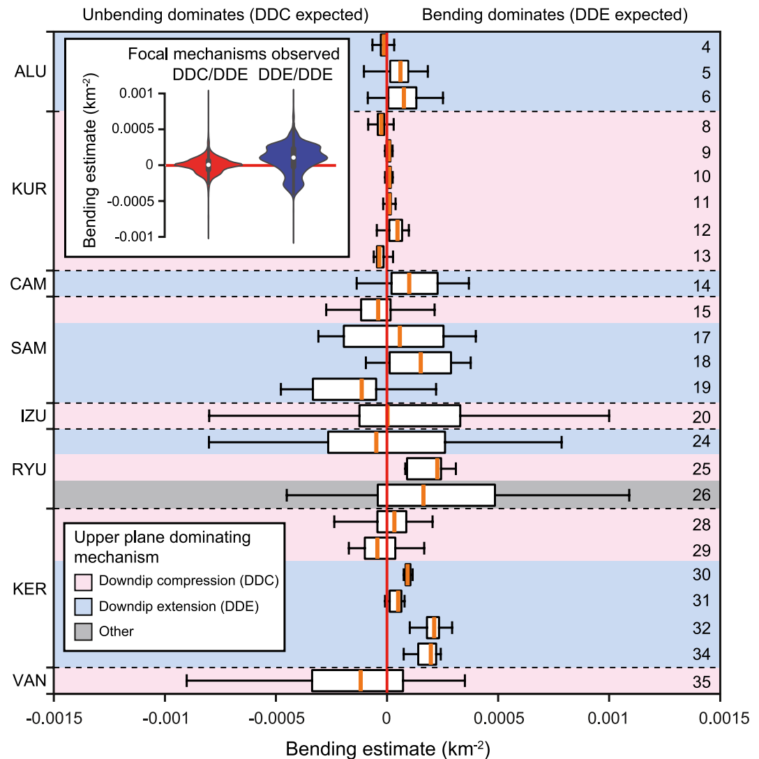
Figure 10. Comparison of focal mechanism information (see Figure 3) to bending estimates for the regions with confirmed Double seismic zone (DSZ) seismicity (Figure 2; Table A2). Shown are boxplots of bending estimates (positive values indicate downward bending, negative values upward bending or “unbending”), in which the orange line represents the median and the white box the inner quartile range of the distribution. The whiskers extend until the furthest data point within another 1.5 inner quartile ranges, outliers are not shown here. Each boxplot represents one region with DSZ and focal mechanism observations, horizontal black lines separate regions belonging to the same slab systems (indicated on the y-axis), the numbers on the right refer to the respective studies (see Figures 2 and 3 and Table A2). Red and blue background color marks regions where downdip compressive or downdip extensive upper plane focal mechanisms are observed, respectively. The inset on the upper left shows a comparison of summed slab (un)bending estimates for all regions with downdip compressive over downdip extensive (DDC/DDE) mechanisms and regions where both planes are downdip extensive (DDE/DDE). For an explanation of the violin plot, refer to the caption of Figure 6. The plot shows that while DDC/DDE regions show bending and unbending in about equal parts, the DDE/DDE regions are significantly shifted toward more plate bending.
