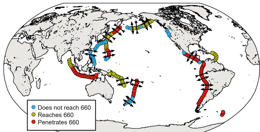
Figure 11. Global compilation of slab extent relative to the 660-km discontinuity, taken from Hu and Gurnis (2020) and based on the tomography models of Li et al. (2008), Obayashi et al. (2013), and Simmons et al. (2012). Intraslab stresses in the double seismic zone, as shown in Figure 3, are plotted on top of the different subduction zones with arrow symbols (two diverging arrows: both planes down-dip extensive; converging over diverging arrow: down-dip compressive over extensive plane).
