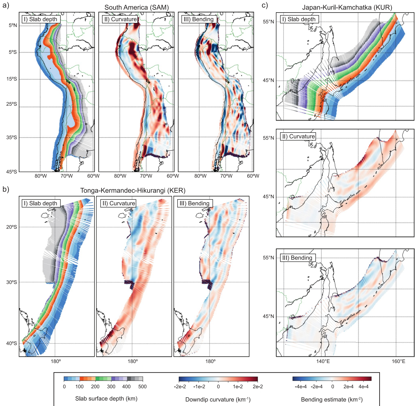
Figure 5. Slab surface depths, downdip curvatures and inferred slab bending/unbending estimates for three selected subduction systems determined from slab2 data. All three properties are shown along the evaluated, trench-perpendicular profiles every 10 km, with along-profile data points about every 2.5 km. Note that negative numbers and blue colors stand for upwards curvature and unbending, whereas positive numbers and red colors represent downward curvature and bending, respectively. For similar plots for the remaining six subduction zones that are shown in Figure 4, please refer to the Supporting Information S1 to this article (Figures S1–S6 in Supporting Information S1).
