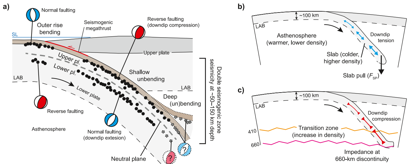
Figure 1. (a) Schematic illustration of double seismic zone (DSZ) seismicity in subduction zones. The two planes of the DSZ are defined by parallel alignments of intraslab earthquakes (black dots). In the outer rise region, the oceanic plate is bent downwards, which leads to extensive focal mechanisms at shallow depth and compressive ones deeper inside the plate. Beyond the megathrust, the slab shape straightens due to unbending, which is thought to cause down-dip compression in the upper plane (pl.) and down-dip extension in the lower plane. Bending stresses are zero along the neutral plane. At greater depth the slab can be further bent or unbent, as indicated by the dashed slab segments. Whether the deep (un)bending causes a reversal in stress and focal mechanisms is not clear. Note that the displayed focal mechanisms are map view projections of LAB, lithosphere asthenosphere boundary; SL, sea level (b, c) In-plane stresses evoked by slab pull (b, down-dip tension) and resistance at the 660-km discontinuity (c, down-dip compression).
