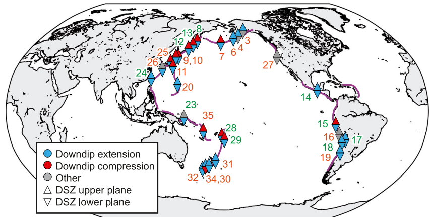
Figure 3. Global survey of focal mechanism data in double seismic zones, numbers next to the symbols refer to the studies listed in Table A1. Orange numbers imply that focal mechanisms were obtained using first motion polarities, green numbers denote studies that used some form of waveform inversion.
