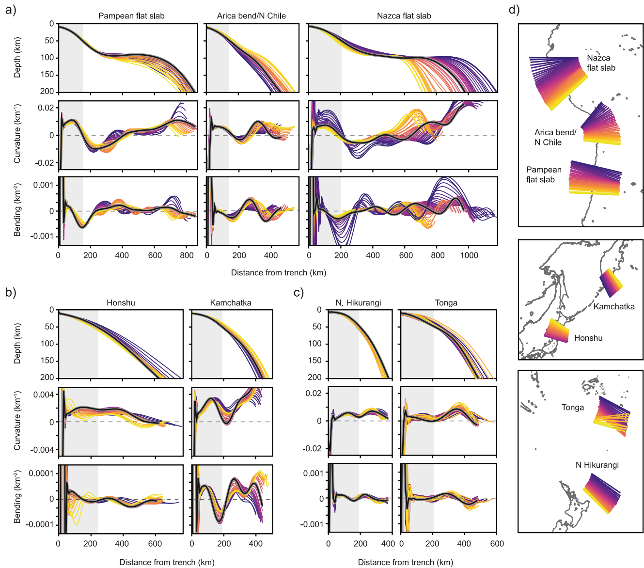
Figure 7. Profiles of slab shape, curvature and bending estimates shown for selected swaths along the South American (a), Japan-Kuril-Kamchatka (b) and Tonga-Kermadec-Hikurangi (c) slabs. Shown are profiles along different swaths (profile position according to color; central profiles of each region shown with thick black lines) in order to capture along-strike variability. For each subfigure, profile positions are shown in (d). Subfigures (a) to (c) consist of two or three columns of plots for the slab geometry (uppermost panel), slab curvature (central panel) and slab bending (lowermost panel). Note that the curvature and bending plots for the Japan-Kuril-Kamchatka slab use different scales compared to the other subfigures due to the much smaller values. The gray shading marks the extent of the uppermost 50 km of each slab, which were not sampled by the violin plots in Figure 6.
