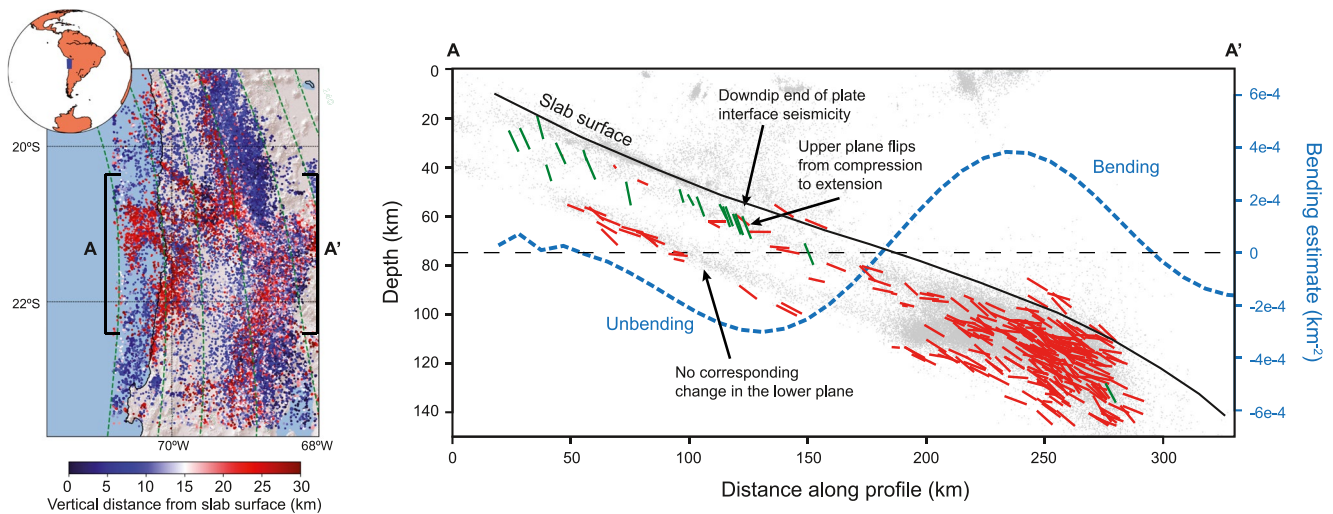
Figure 12. (Left) Earthquake epicenters from the years 2007–2014 taken from the Northern Chile earthquake catalog of Sippl et al. (2018), color-coded by their distance to the slab surface. Blue colors denote upper plane, red colors lower plane events. Black brackets show the swath that is plotted as an E-W profile section in the right subplot (Right) Intraslab stress orientations in Northern Chile, plotted atop hypocenters from within 1 degree of the profile center at 21.5°S (see left subplot). Red and green bars show the orientation of tensional axes (T axes) of earthquake focal mechanisms from Sippl et al. (2019) within the same swath. Note that the length of each bar indicates whether the T axis is mostly parallel to the profile plane (long bars) or perpendicular to it (point). Green color is chosen when a tensional axis deviates from the slab dip by more than 45°, which is the case when events are downdip compressive. The blue line shows the bending/unbending estimates from the profile through the slab2 data set that is located closest to the shown seismicity cross section (see Figure 5), the black line is the slab surface according to Sippl et al. (2018).
