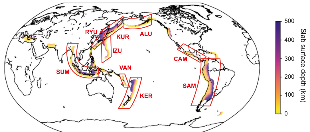
Figure 4. Slab surface depths of all oceanic slabs contained in the slab2 data set (Hayes et al., 2018). The nine large slab systems analyzed in the present study are marked by red frames, and their three-letter abbreviations are given. ALU, Alaska-Aleutian; CAM, Central America; IZU, Izu-Bonin-Mariana; KER, Tonga-Kermadec-Hikurangi; KUR, Japan-Kuril-Kamchatka; RYU, Ryukyu-Nankai; SAM, South America; SUM, Andaman-Sumatra-Sunda; VAN, Vanuatu.
