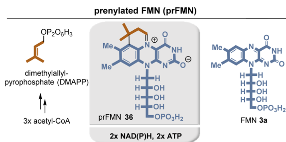
Fig. 5 Summary of prenylated flavin mononucleotide (prFMN) biosynthesis with building blocks marked in sienna and blue including positions where they end up in prenylated flavin mononucleotide (prFMN) 36. Coenzyme-dependent enzymes (refer to the synthesis of DMAPP by the mevalonate pathway): NAD(P)H: HMG-CoA reductase; ATP: mevalonate kinase and phosphomevalonate kinase.
