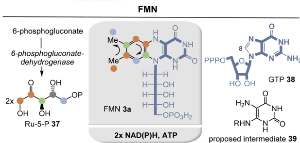
Fig. 4 Structures of pterin 34, isoalloxazine 35 and prFMN 36 (top). Summary of flavin biosynthesis with building blocks marked in sienna and blue including positions where they end up (bottom). Coenzyme-dependent enzymes: NAD(P)H: 6-phosphogluconate-dehydrogenase and 5-amino-6-(5-phosphoribosylamino)uracil reductase ( ribD ); ATP: riboflavin kinase ( ribF ); biosyntheses in fungi and bacteria only differ in timing of individual steps.
