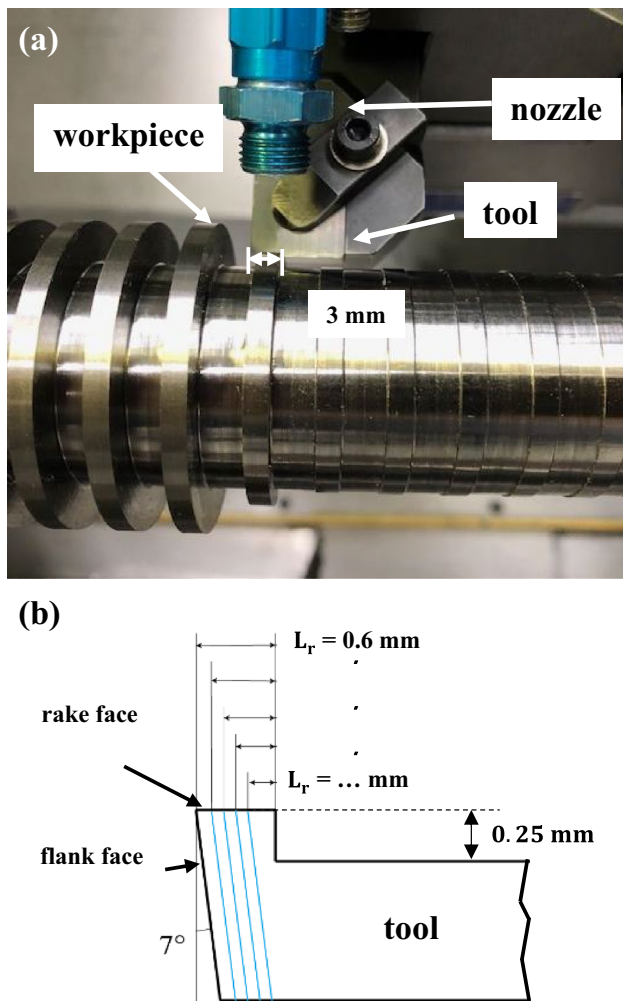
Fig. 4 a Experimental setup of quasi-orthogonal turning; b Preparation of restricted tools for the cutting experiments
