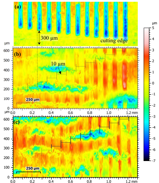
Fig. 7 Topography images of the inverse micro texturing on the backside of the chip for Ti6Al4V and an uncut chip thickness of h=0.2 mm and v_c=120 m/min. a Dry machining l_c=300 \mu\text{m} b wet machining l_c=290 \mu\text{m}
