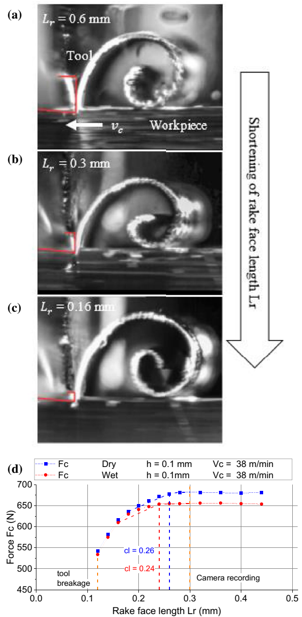
Fig. 12 a–c High speed images of orthogonal cutting of Ti6Al4V with v_c = 38 m/min, h = 0.1 mm and b = 3 mm for dry process with different rake face lengths L_r = 0.6 mm; 0.3 mm; 0.16 mm); d measured cutting forces (dry and wet p = 30 bar); drop of cutting forces in dry and wet cutting (mean values of three processes)
