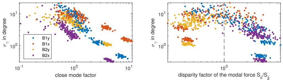
Fig. 15 Standard deviation of the direction angle \gamma of the mode shape as a dependence of the close mode factor e and the disparity factor d on the modal forces.
