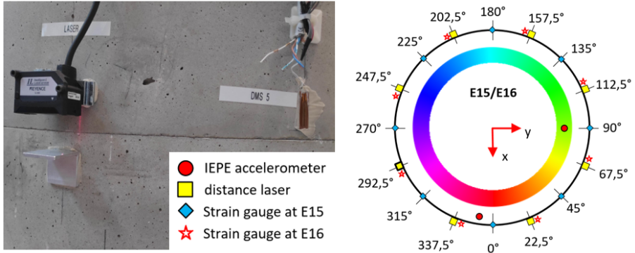
Fig. 5 Displacement laser sensors and strain gauges at the joint between segment E15 and E16. The colour gradient in the right shows the colours for the different sensor positions for Figure 6.
