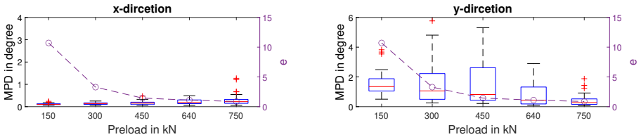
Fig. 19 Distribution of the MPD of the complex mode shape B1X of the SSI as well as the close mode factor e as a function of the preload levels separated according to measurement directions.
