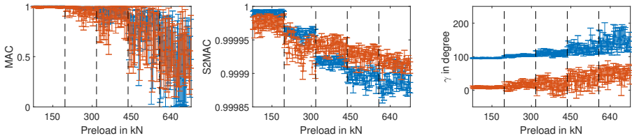
Fig. 11 Influence of the preload on the MAC, S2MAC and direction angle \gamma of the first bending mode pair identified with BAYOMA. Red is the B1X, blue the B1Y.
