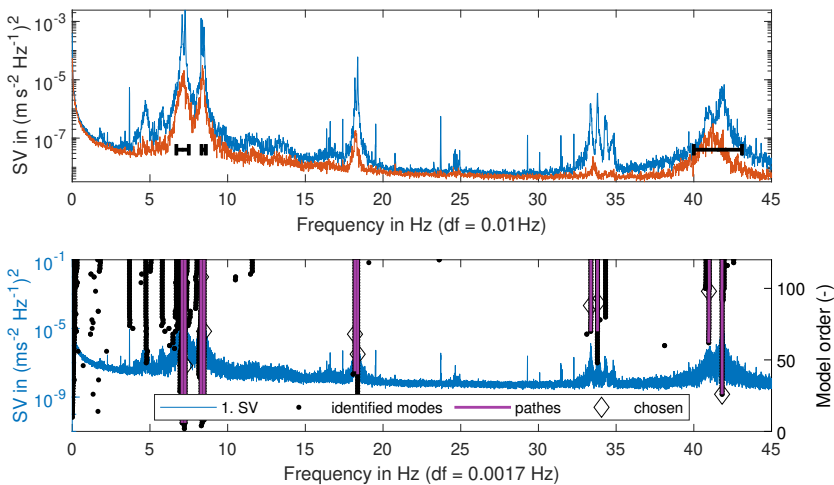
Fig. 7 Top: Two highest singular values (SV) of the averaged spectral matrix. The identification range of BAYOMA is marked with black lines. Bottom: Stabilisation diagram from the SSI-COV based on an unaveraged spectral matrix. The data is from a measurement at a preload level of 150 kN.
