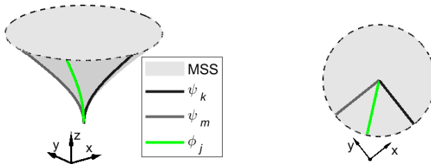
Fig. 3 Visualisation of the mode subspace (MSS) from the first bending mode pair [\psi_k \psi_m] of a cantilever structure. Another possible mode shape \phi_j is shown in green.
