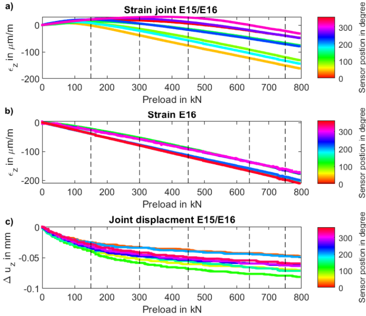
Fig. 6 Dependence of strain and displacement in z-direction on the preload
