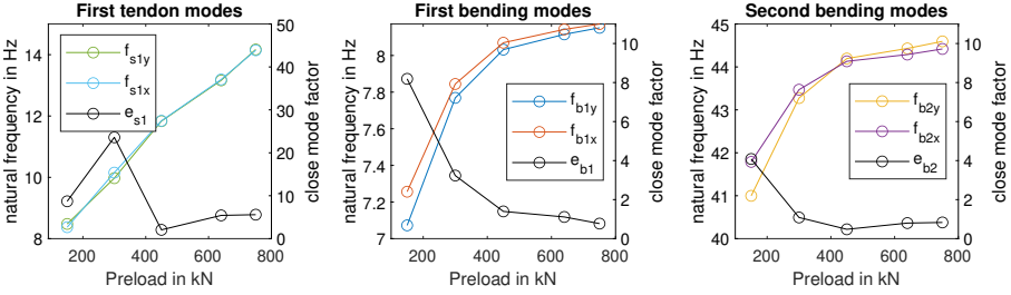
Fig. 9 The natural frequencies identified with BAYOMA and the close mode factor as a dependence on the preload levels.
