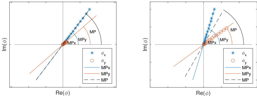
Fig. 17 Illustration of two B1X modes of two different preload levels in the complex plane separated according to measurement directions. On the left for a mode at a preload level of 150 kN, that the MP is almost identical to the MP in the dominant direction. On the right for a mode at a preload level of 750 kN, where two lines exist in the complex plane.
