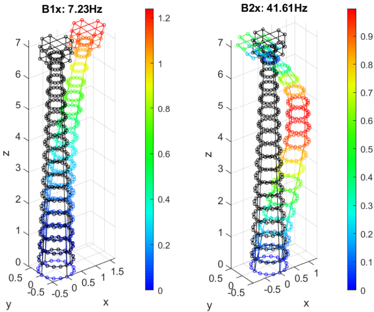
Fig. 8 Mode shape of the first two bending modes in the x -direction at 150 kN preload identified with BAYOMA.
