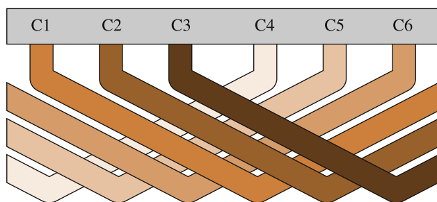
Fig. 8 Excerpt from a hairpin end winding region
